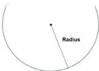
Centrifugal force. Illustration: FFWPU
