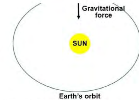
Gravitational and centrifugal force. Illustration: FFWPU
