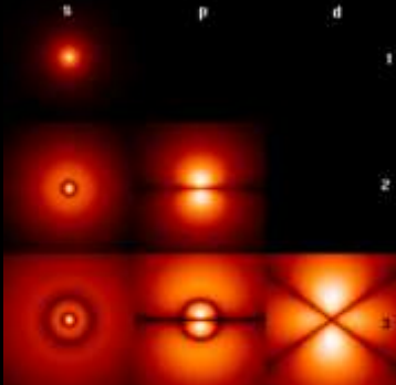
Electron/ Positron
