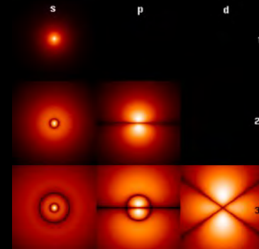
Electron/ Positron
